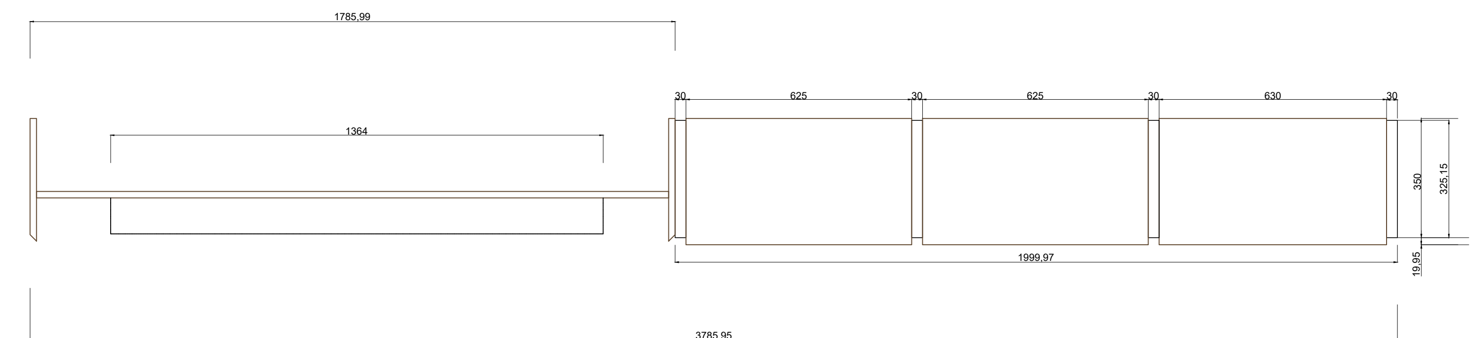
MOBİLYA DETAY PLAN 1/10
